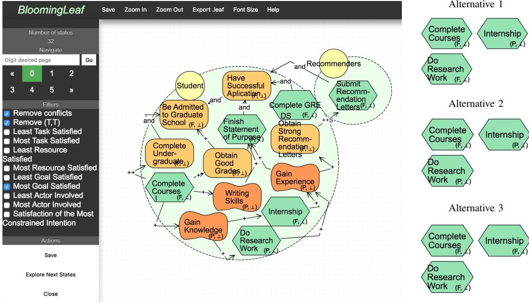
(a) Screenshot of the Next States pop-up window in BloomingLeaf, showing the GRAD model on the centre canvas with three filters selected.
